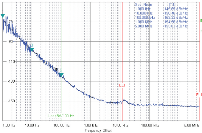
Typical Phase Noise for DOCSC022V-024.576M
