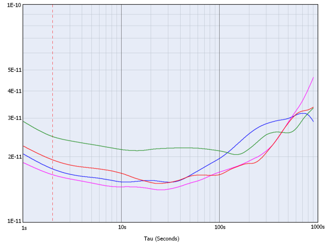
Allan Deviation DOCSC022F-024.576M
