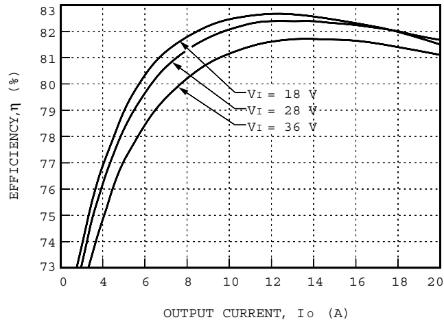
Figure 9. Typical JC100A Converter Efficiency vs. Output Current at Room Temperature
