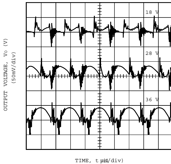
Figure 10. Typical JC100A Output Ripple Voltage at Room Temperature and 20 A Output
