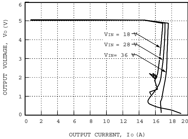
Figure 5. Typical JC075A Output Characteristics at Room Temperature.
