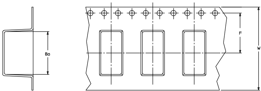
EMBOSED CARRIER TAPE TYPE 'A'
