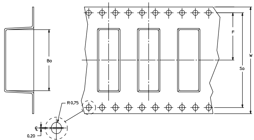
EMBOSED CARRIER TAPE TYPE 'B'
