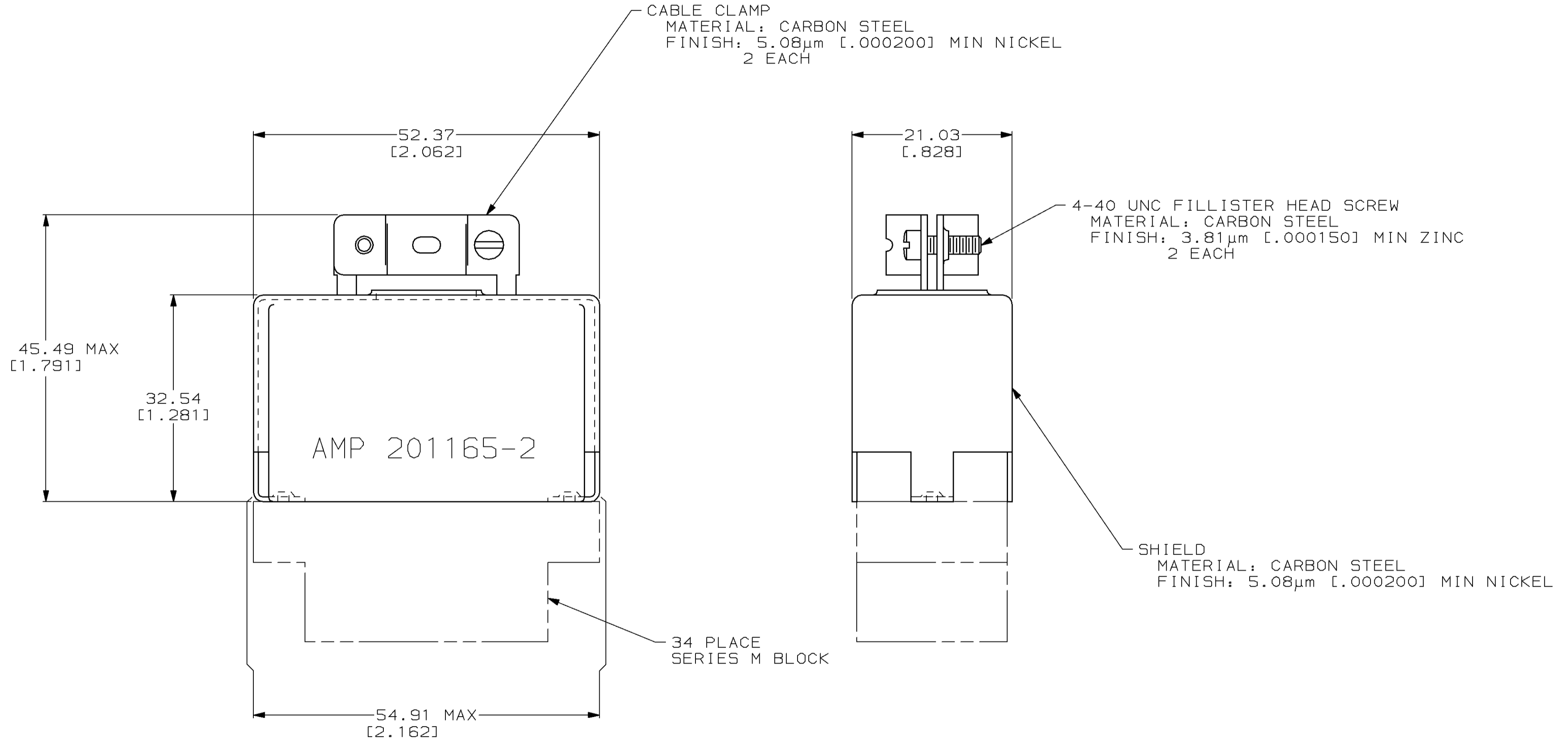
ASSEMBLED VIEW
