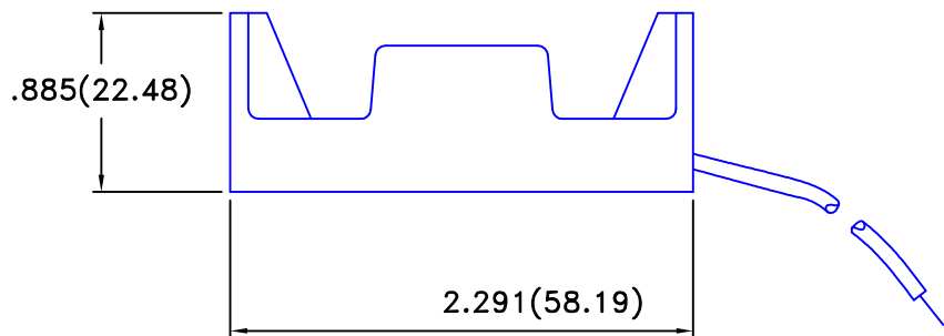
Wire Leads Shown
