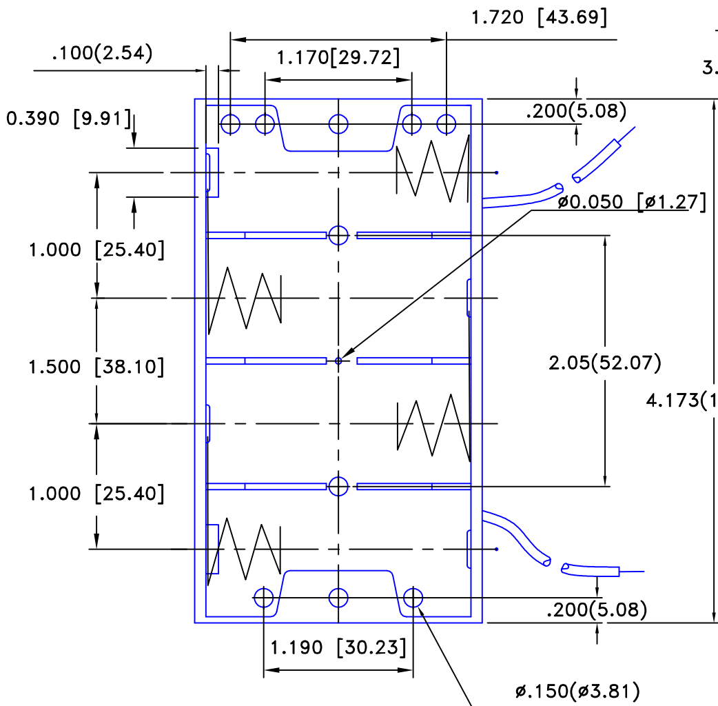
Wire Leads Shown
